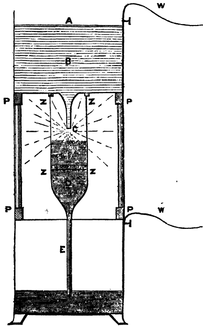
Fig. 189. Way's Mercurial Electric Lamp. A. Upper iron cistern containing B, the mercury, which falls slowly, in a fine stream, through the minute aperture, C, on to a little cup not shown, because invisible when the light is produced, and placed in the glass tube z z z z, connected with the lower iron cistern, E. The two metallic cisterns are cut off from conducting communication with each other by the non-conducting material inserted at the pillars P P, P P. W, W. Wires passing to the voltaic battery.
